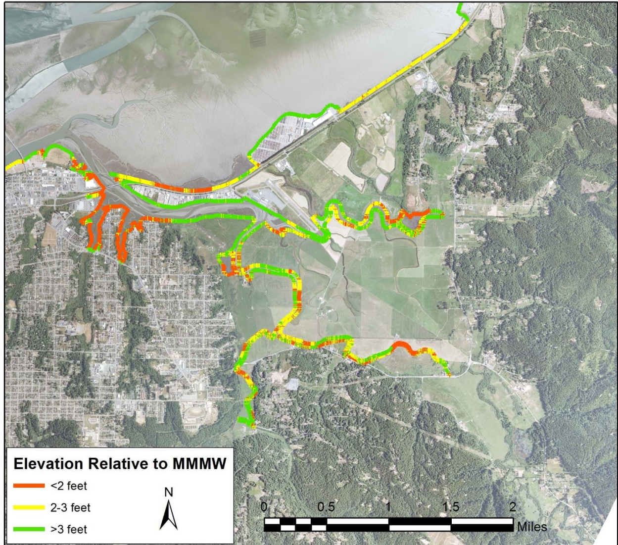
Figure 8. . Shoreline elevation above the MMMW elevation of 7.7 ft (NAVD 88): red <2 ft, yellow = 2-3 ft, and green > 3 ft, on Eureka Slough and Arcata Bay (Laird 2013).
