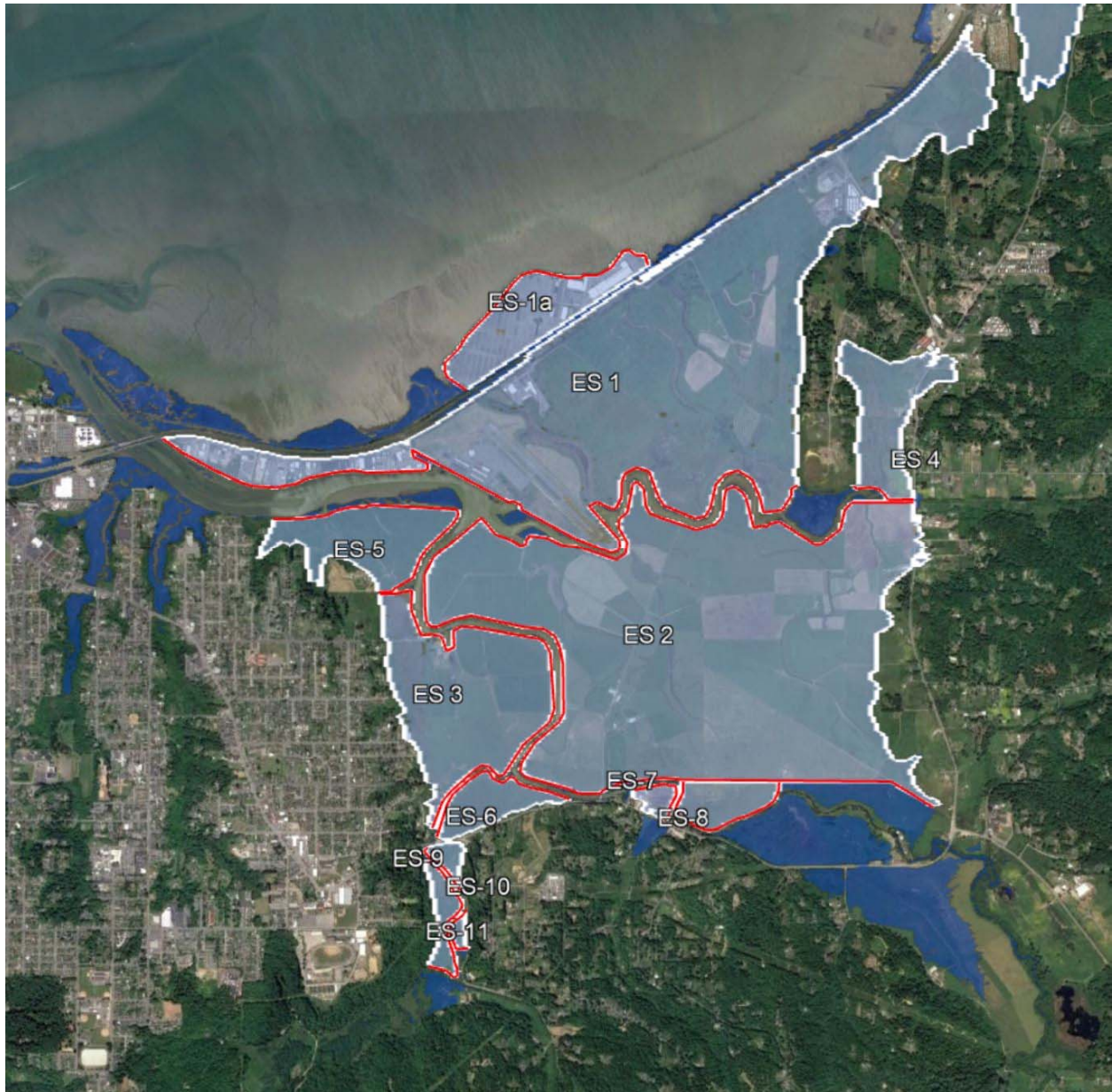
Figure 4. Diked shoreline hydrologic sub-units: Eureka Slough (ES), diked shoreline reaches (red), and potential MAMW inundation area (blue).
