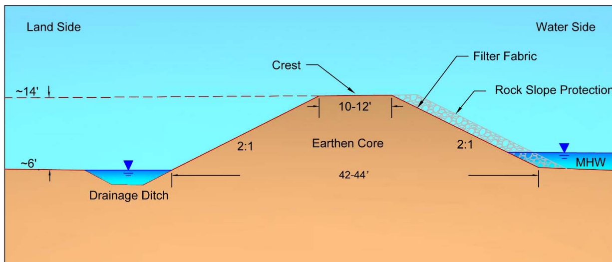
Figure 21. Typical dike features, drainage ditch, earthen core, 2:1 slopes, crest height equal of 14 feet (MAMW elevation by 2100) width for vehicular access, and rock slope protection.
