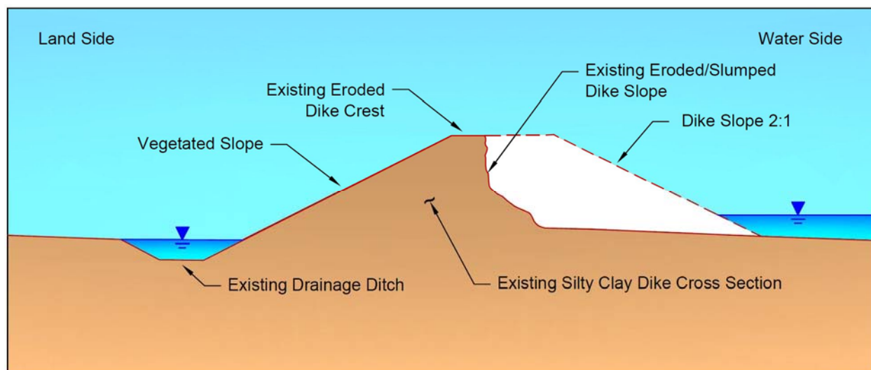
Figure 17. Eroded water side of an earthen dike illustrating typical dike features and the reduction in crest width.
