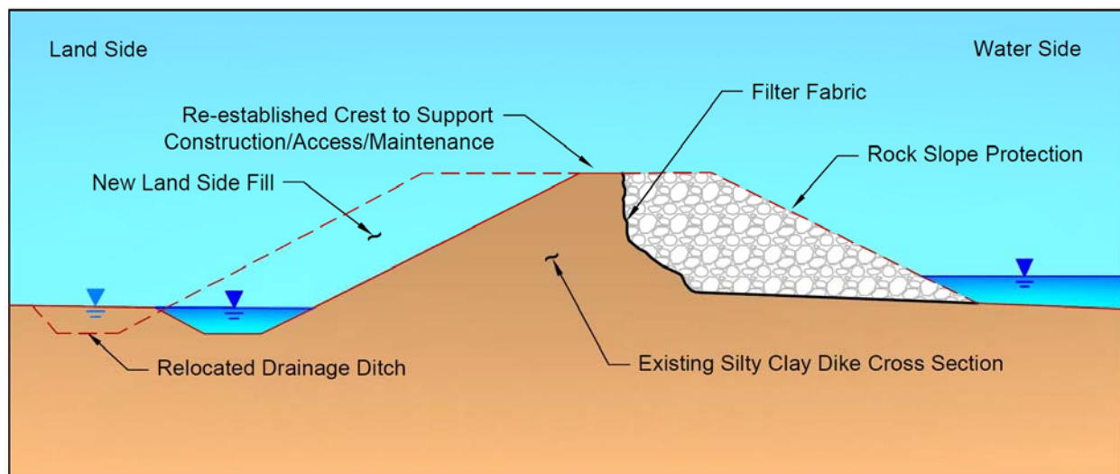
Figure 18. Modification of original dike design by rebuilding the dike on the landward side of the existing dike.
