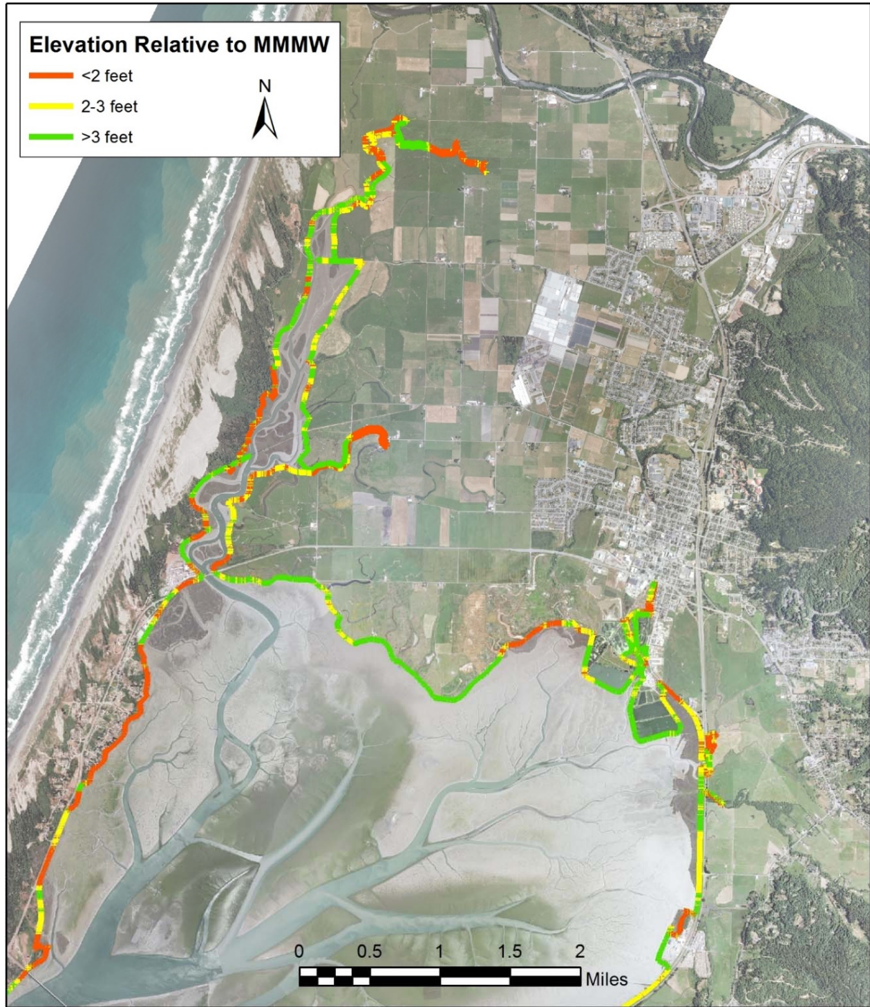
Figure 7. Shoreline elevation above the MMMW elevation of 7.7 ft (NAVD 88): red <2 ft, yellow = 2-3 ft, and green > 3 ft, on Mad River Slough and Arcata Bay (Laird 2013).
