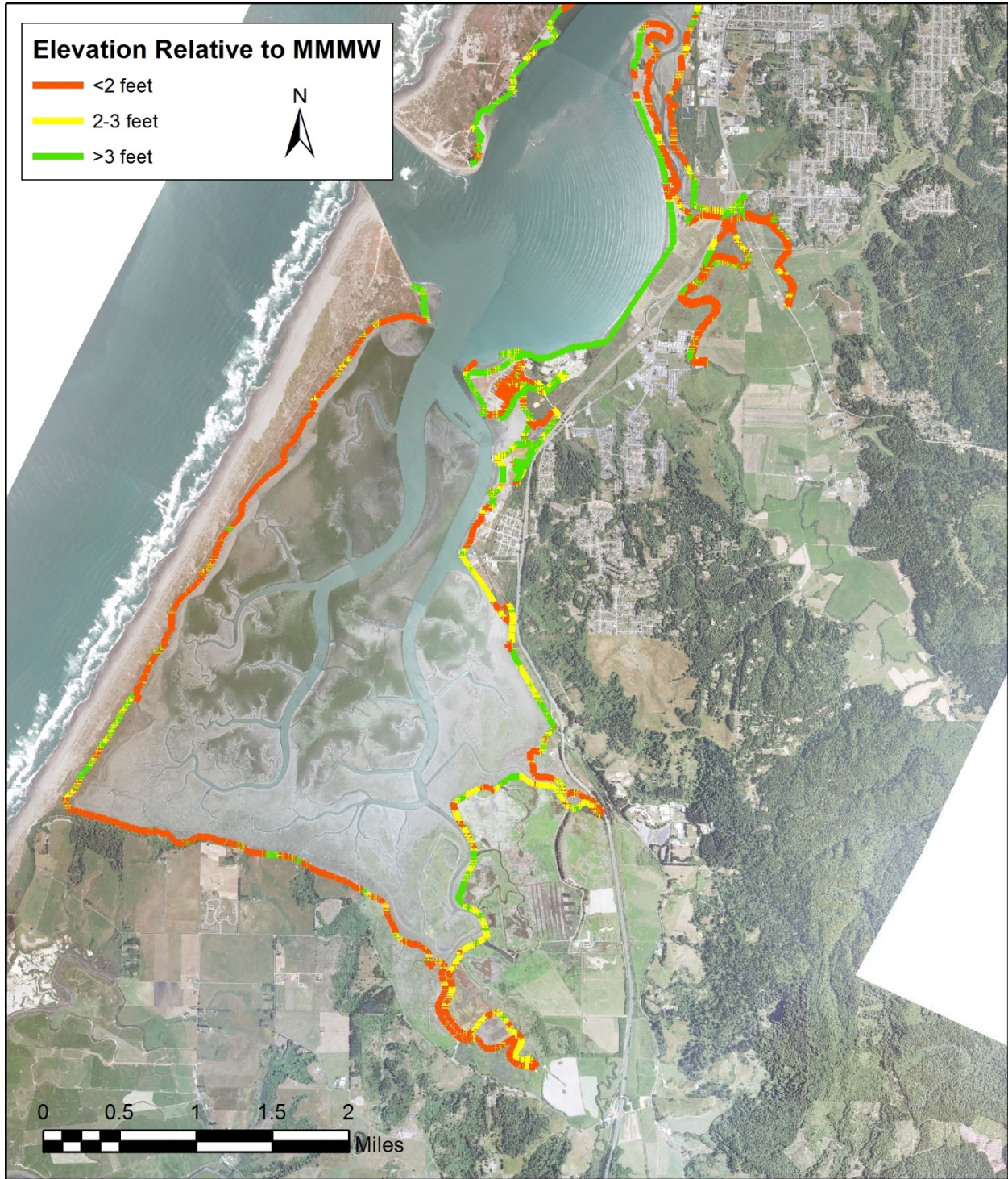
Figure 9. Shoreline elevation above the MMMW elevation of 7.7 ft (NAVD 88): red <2 ft, yellow = 2-3 ft, and green > 3 ft, on Elk River Slough and South Bay (Laird 2013).
