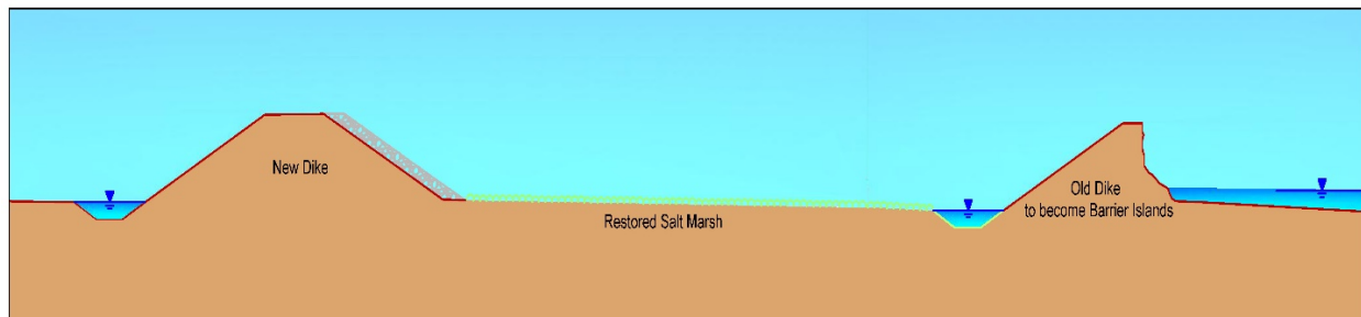
Figure 20. Relocated dike with former dike barrier island feature and restored salt marsh natural infrastructure for new dike.
