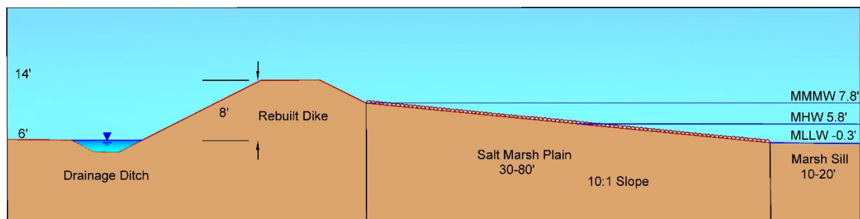
Figure 19. Natural shoreline infrastructure, a combination of a marsh sill and salt marsh plan.
