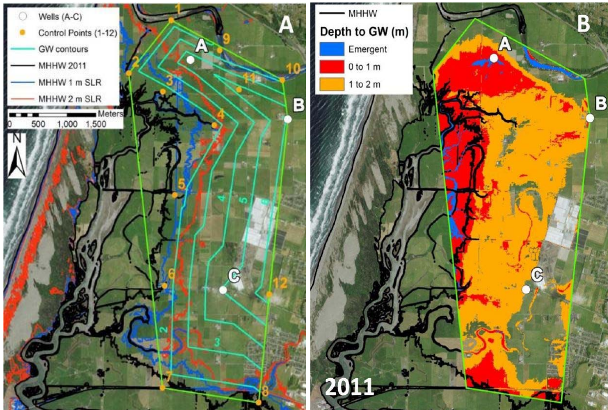
Figure 13.. From Hoover 2015, as based on Willis 2014. Fresh groundwater floats on higher-density seawater, and the average elevation of the water table would be above MSL 3.4 ft. MHHW is 6.5 ft.
