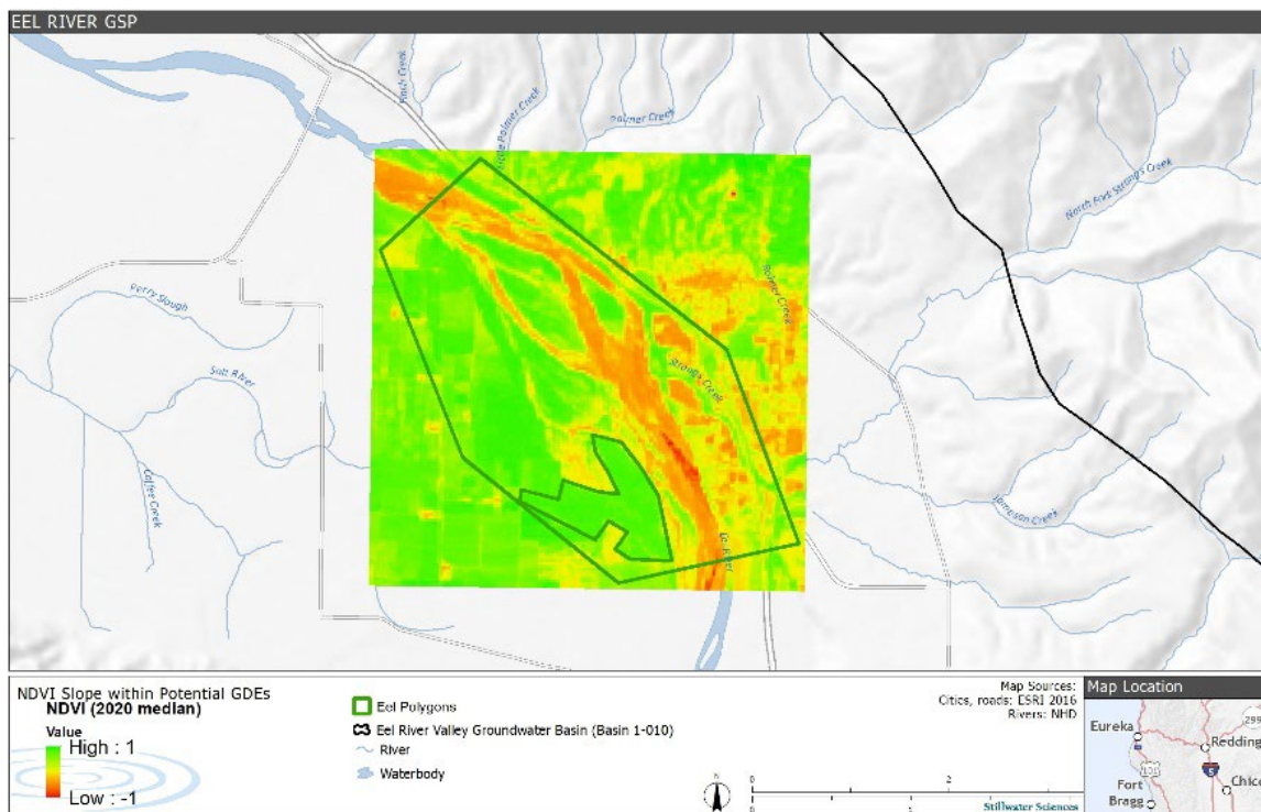
Figure 4. Median summer 2020 NDVI near Fortuna, CA. The smaller polygon outlines the potential GDE discussed in the CDFW comments.
