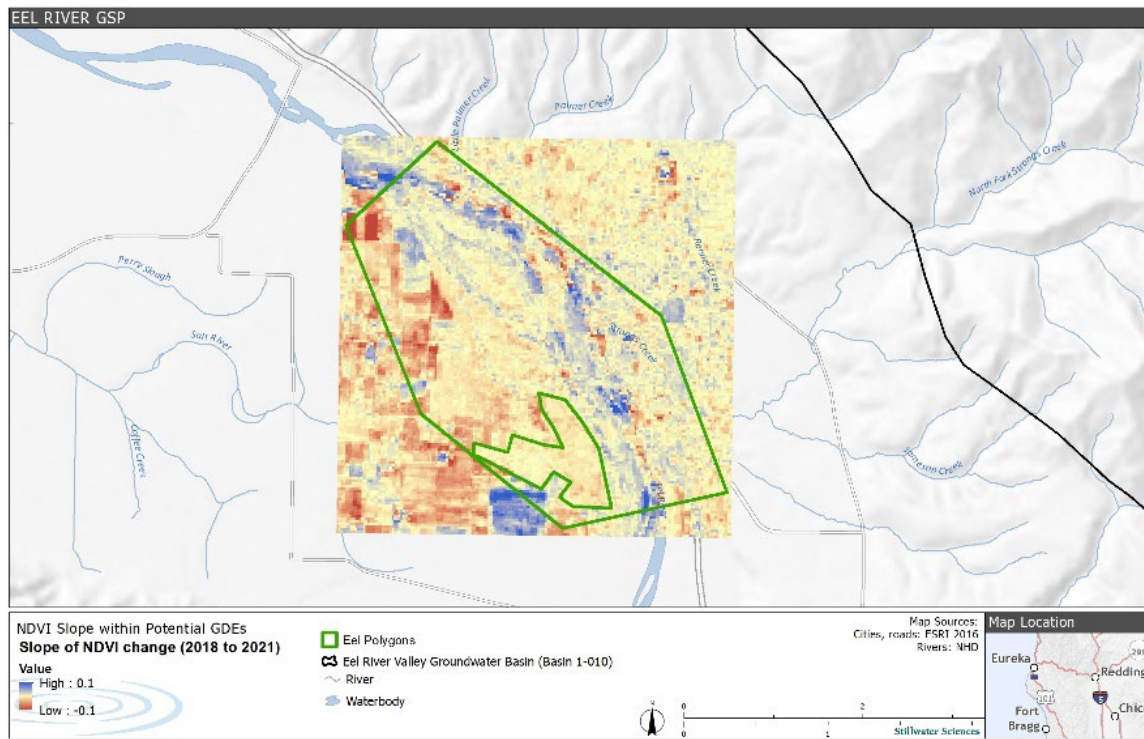
Figure 1. Slope change of NDVI from 2018-2021 near Fortuna. The smaller polygon outlines the potential GDE discussed in the CDFW comments
