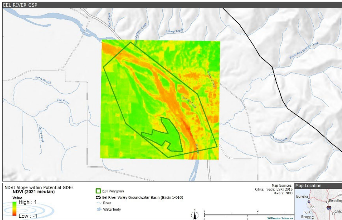
Figure 5. Median summer 2021 NDVI near Fortuna, CA. The smaller polygon outlines the potential GDE discussed in the CDFW comments.
