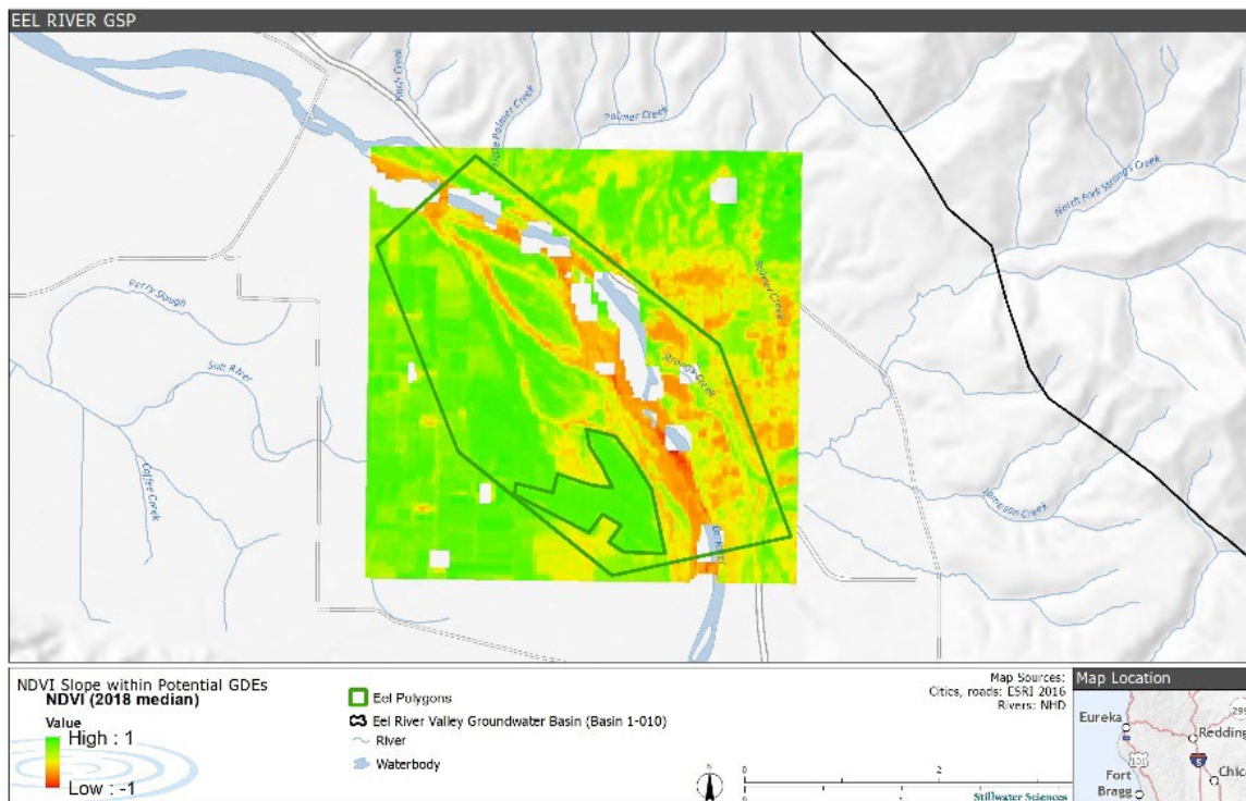
Figure 2. Median summer 2018 NDVI near Fortuna, CA. The smaller polygon outlines the potential GDE discussed in the CDFW comments.
