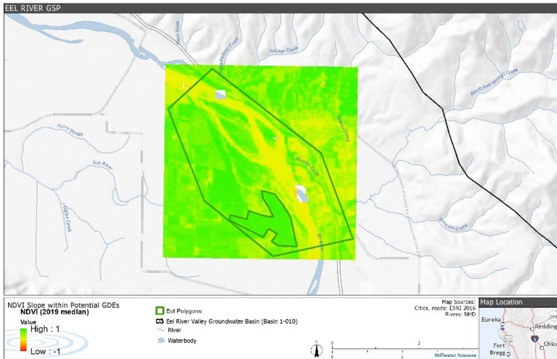
Figure 3. Median summer 2019 NDVI near Fortuna, CA. The smaller polygon outlines the potential GDE discussed in the CDFW comments.
